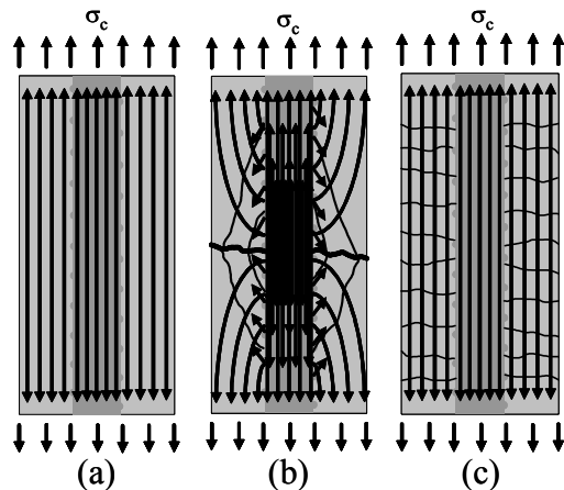
Figure 2. (a) Composite before matrix cracking (b) R/C after cracking (c) R/ECC after cracking
