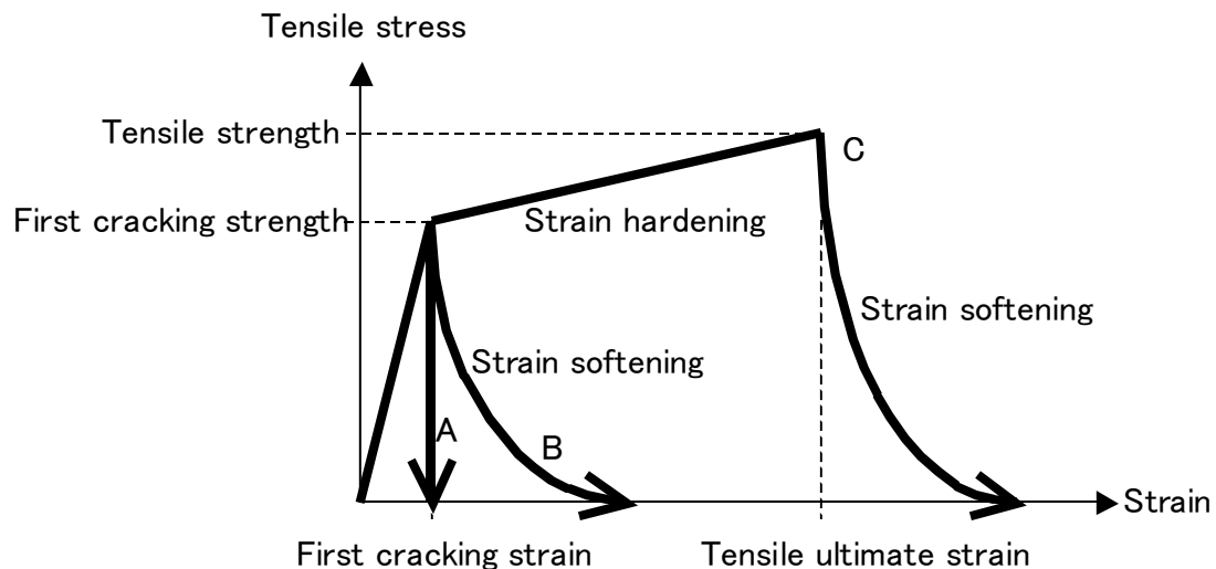
Figure 2 Definition of A: brittle, B: quasi brittle, and C: ductile behavior as well as strain softening and strain hardening under uniaxial tensile loading.
